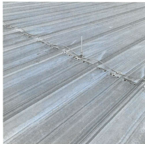
Screws rusted; rubber washer deteriorated. Remove and install new fasteners with new butyl tape.
