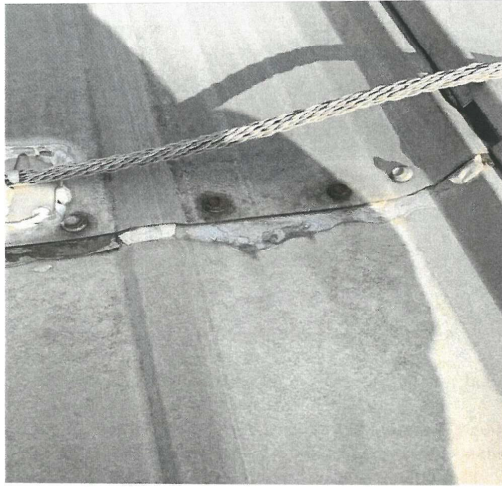
Deteriorating butyl in laps. Multiple laps are beginning to fail. New butyl tape needed to ensure the life of the roof.
